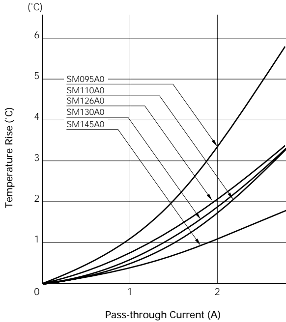
Temperature Rise
